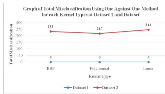
Fig. 2. Graph of total misclassification using One Against One method for each kernel type at dataset 1 and dataset 2
