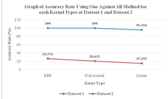
Fig. 3. Graph of accuracy rate of One Against All method for each kernel type at dataset 1 and dataset 2
